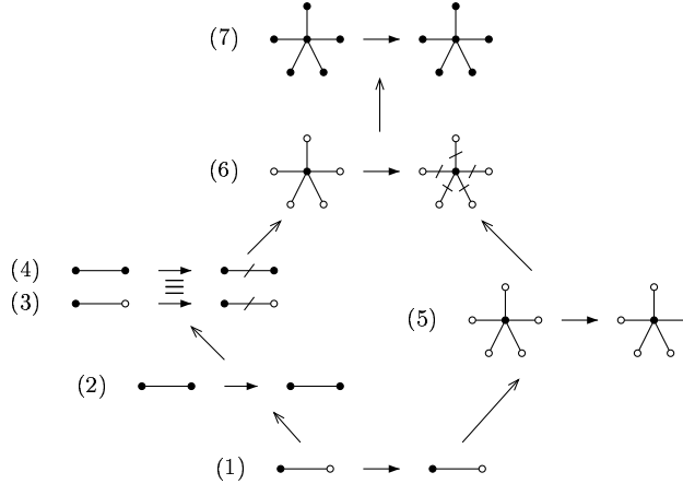
Figure 6: A hierarchy of local computations models described by the different kinds of relabeling rules they use.
