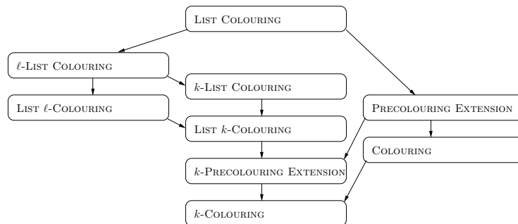
Figure 1. Relationships between COLORING and its variants as shown in [27]. An arrow from one problem to another indicates that the latter is a special case of the former; k and \ell are any two integers for which \ell \geq k .
